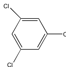
1,3,5-triklorobentzenoa
